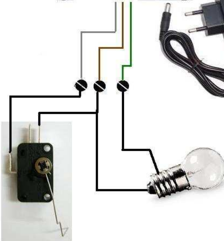
Coin switch or push button
